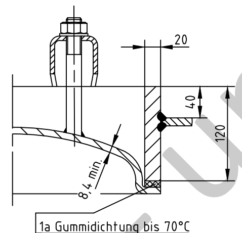
Detail X
